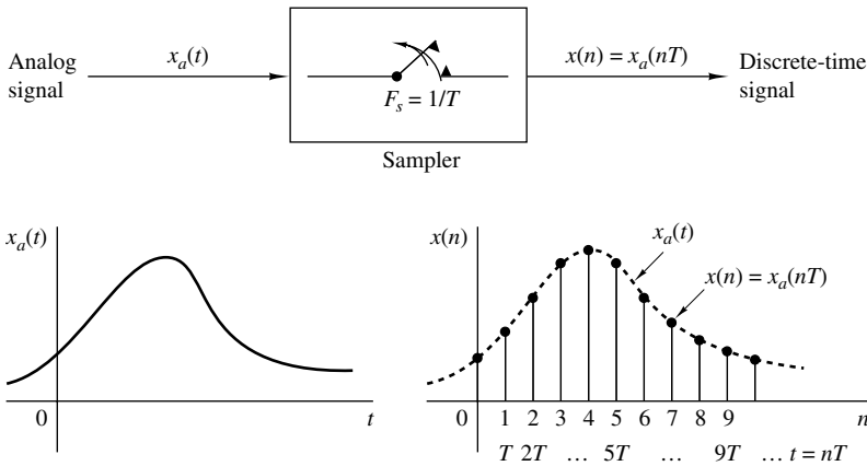
Figure 4.3 Periodic sampling of an analog signal.
