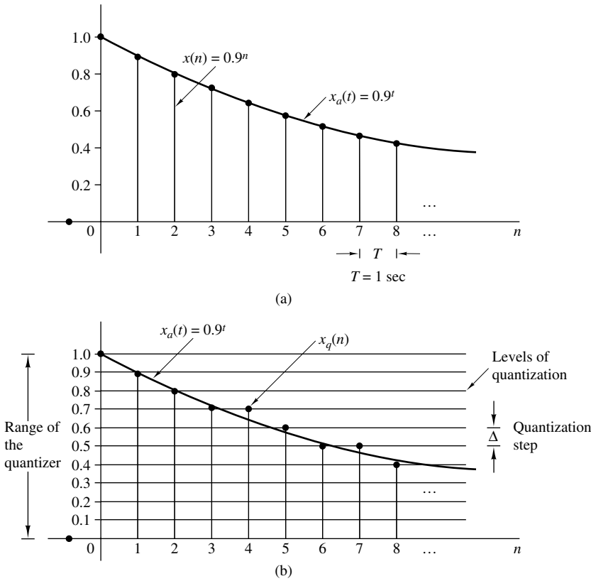
Figure 4.7 Illustration of quantization.
