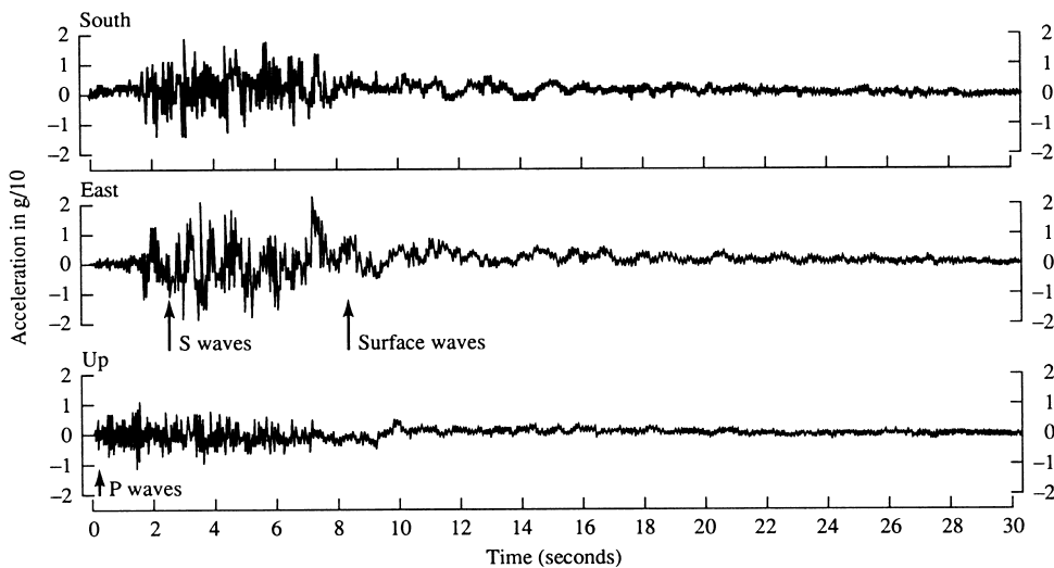
Figure 2.1 Three components of ground acceleration measured a few kilometers from the epicenter of an earthquake. (From Earthquakes , by B. A. Bold, ©1988 by W. H. Freeman and Company. Reprinted with permission of the publisher.)
